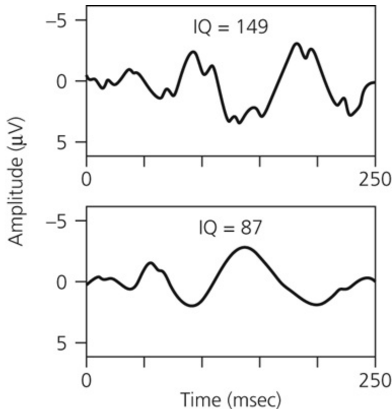
String length. Typical evoked potentials from a person with a high IQ (top) and a person with a low IQ (bottom).
