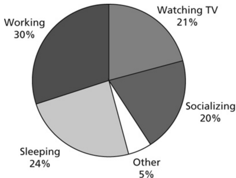
Pie chart. Showing percentages of time spent by a group of people in various types of activities.
