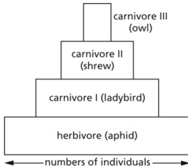
Pyramid of numbers. A woodland food chain.
