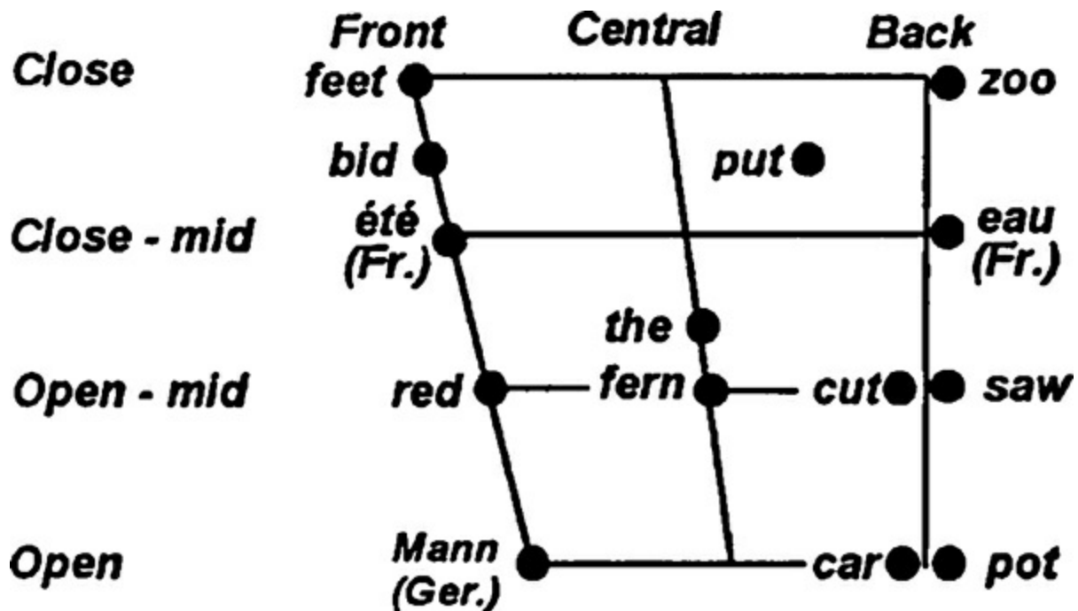
Vowel quadrilateral
